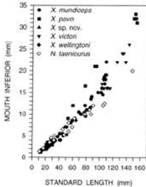
Fig. 4. The relationship between the inferior placement of the mouth and standard length for the eastern Pacific razorfishes.
