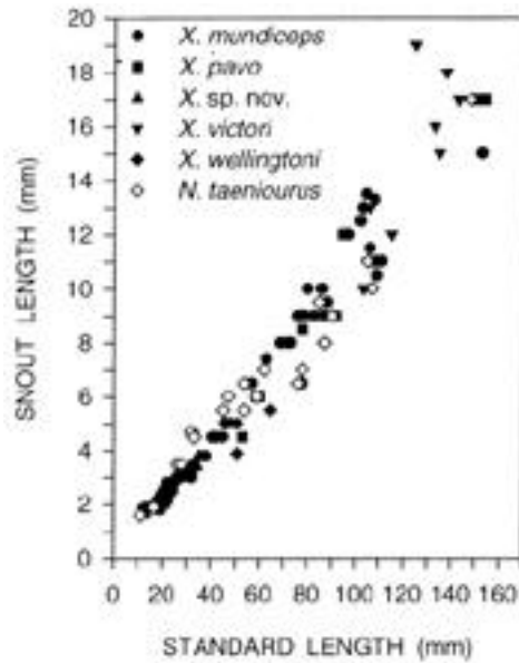
Fig. 2. The relationship between snout length and standard length for the eastern Pacific razorfishes.
