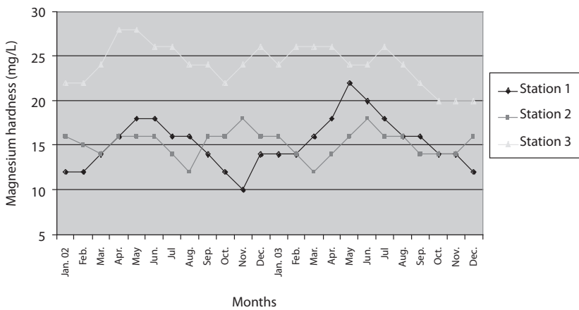
Fig. 10. Monthly mean variations of magnesium hardness in Oyun Reservoir.
